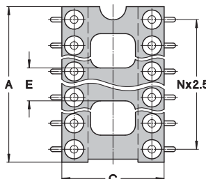
INSULATOR
