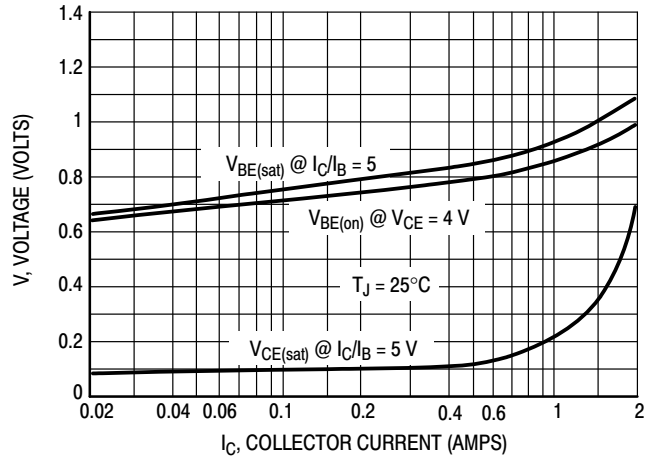
Figure 2. "On" Voltages
