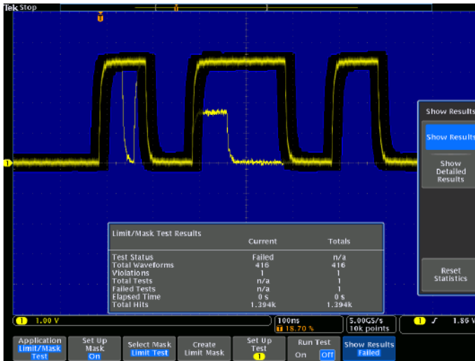
Limit Test showing a mask created from a golden waveform and compared against a live signal. Results showing statistical information about the test are displayed.
