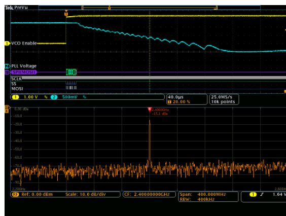
4. The PLL eventually settles on the correct 2.400 GHz frequency about 320 µs after the VCO was enabled.
