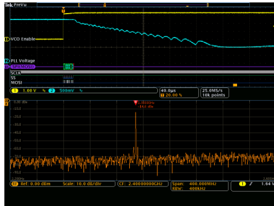
3. Spectrum Time is moved another 160 µs to the right. At this point the spectrum shows that the PLL has actually overshoot the correct frequency and gone all the way down to 2.3888 GHz.
