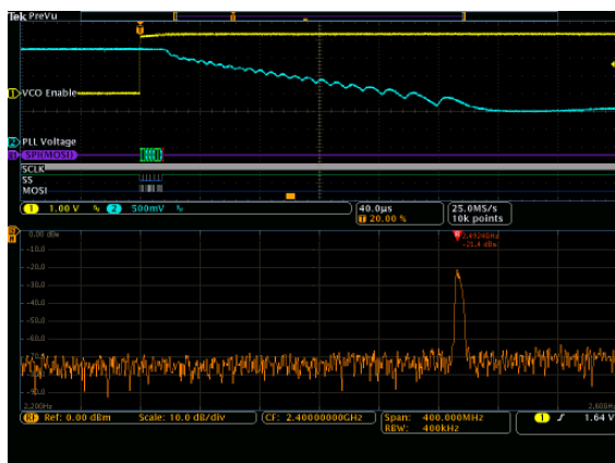
2. Spectrum Time is moved about 90 µs to the right. At this point, the spectrum shows that the PLL is in the process of tuning to the correct frequency (2.400 GHz). It has made it down to 2.4924 GHz.
