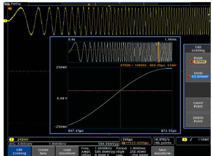
Arbitrary waveform editor showing the point-by-point editor.
