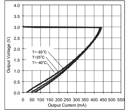
Fig.52 OCP Threshold
