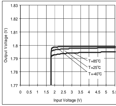
Fig.2 Line Regulation
