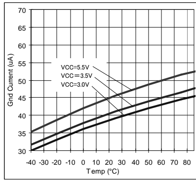
Fig.54 IGND - Temp
