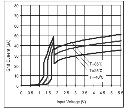
Fig.3 Circuit Current
