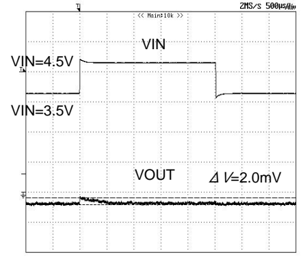
Fig.14 Transient_response (Ta=85°C)
