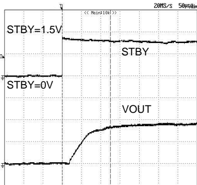
Fig.15 START_UP (Ta=-40°C)
