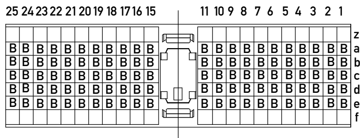
CONTACT LAYOUT
