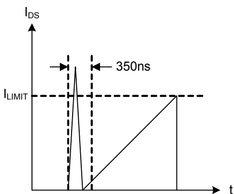
Figure 5: Leading-Edge Blanking
