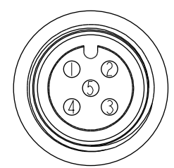
Conn. 1 & Conn. 2 Pin Assignments Front View
