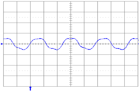
Fig. 6.0V.13: Output voltage ripple (50 mV/div.) at full rated load current into a resistive load with C_o = 10 \mu\text{F} tantalum + 1uF ceramic and V_{in} = 24 \text{ V} . Time scale: 1 \mu\text{s}/\text{div} .
