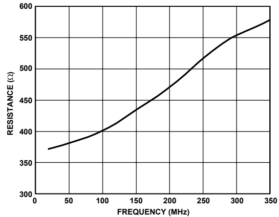
Figure 44. The Shunt Input Resistance vs. the Frequency of the AD9864's IF1 Input
