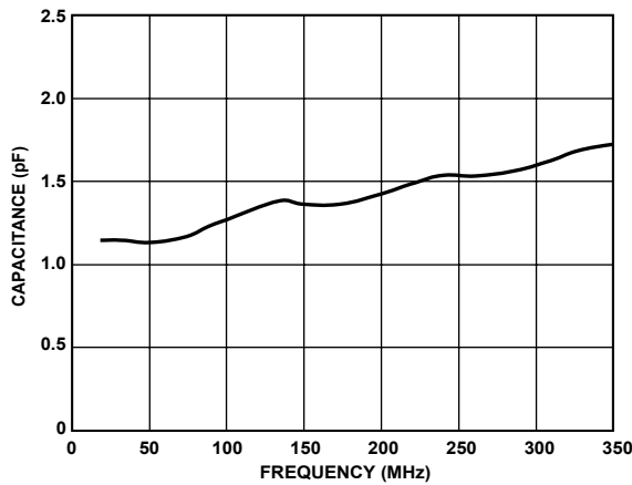
Figure 45. The Shunt Capacitance vs. the Frequency of the AD9864's IF1 Input
