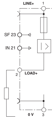
Figure 7 EC 1 12DC... S-C signal inputs/outputs
