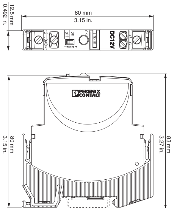
Figure 1 Dimensions
