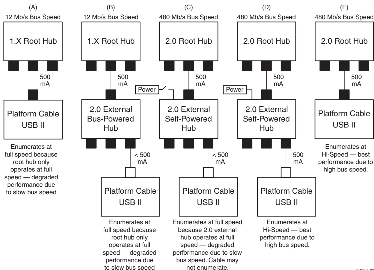
Figure 30: Platform Cable USB II Performance with Various Hub Types
