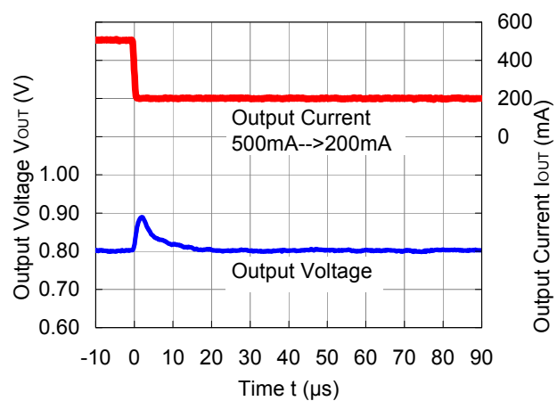
RP504x081x ( V_{IN} = 3.6\text{ V} )
