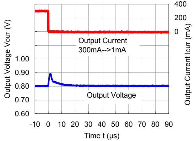
RP504x081x (V IN = 3.6 V) MODE = "H" Forced PWM Control
