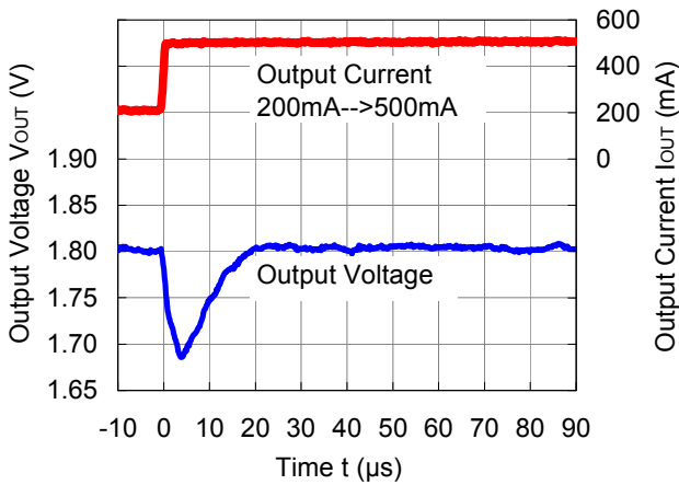
RP504x331x ( V_{IN} = 5.0\text{ V} )
