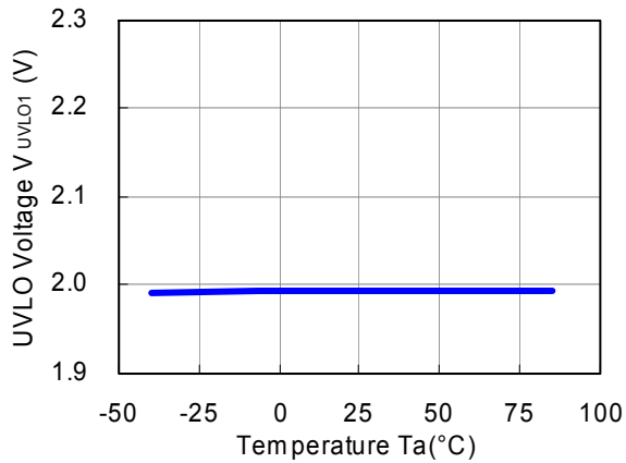
UVLO Detector Threshold Voltage
