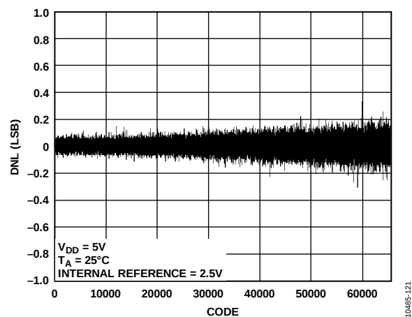
Figure 18. AD5686R DNL
