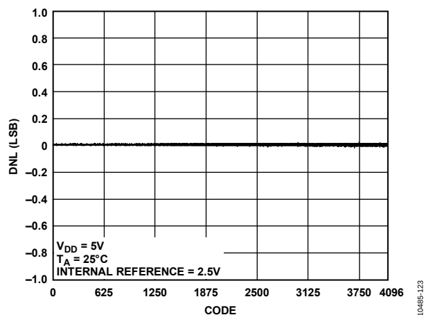
Figure 20. AD5684R DNL
