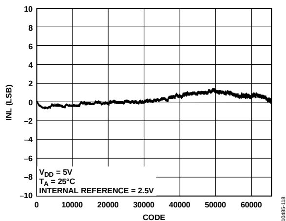
Figure 15. AD5686R INL
