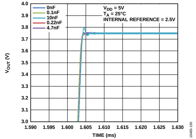
Figure 46. Settling Time vs. Capacitive Load
