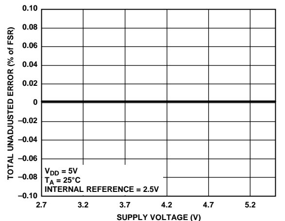
Figure 29. TUE vs. Supply, Gain = 1
