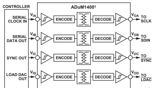
Figure 62. Isolated Interface
