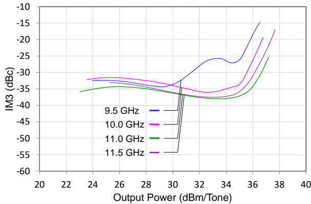
IM3 vs. Pout/Tone vs. Frequency
