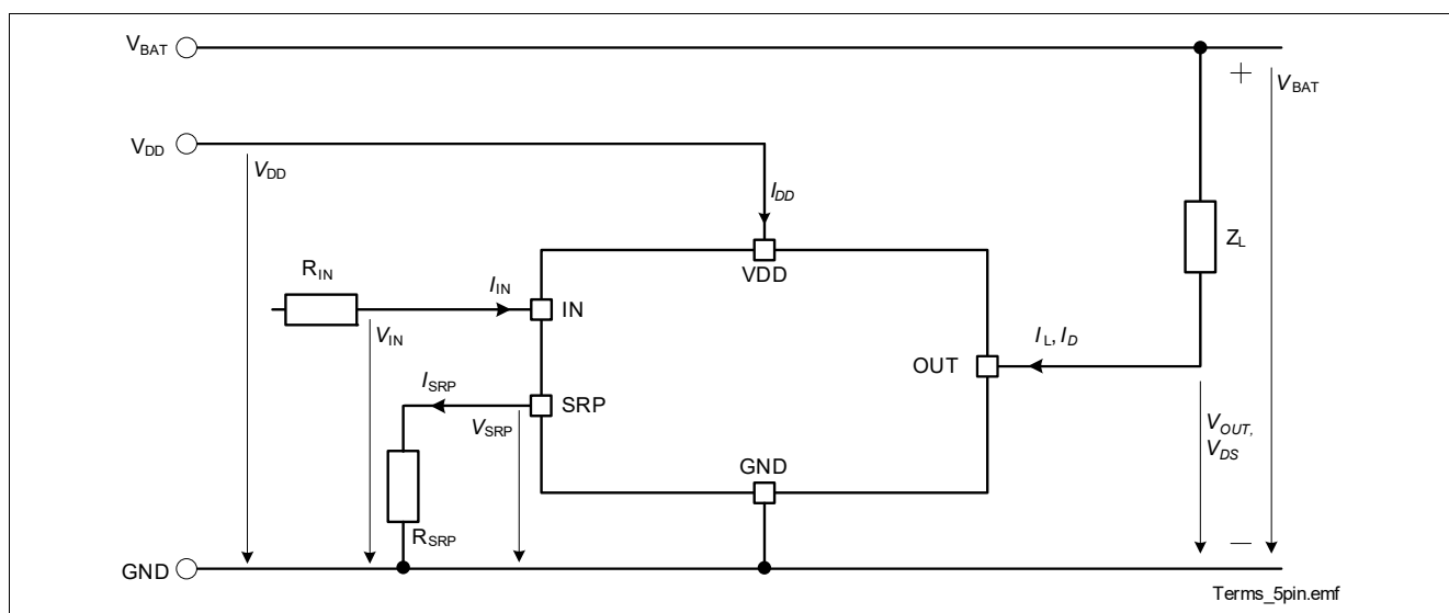
Figure 3 Naming Definition of electrical parameters
