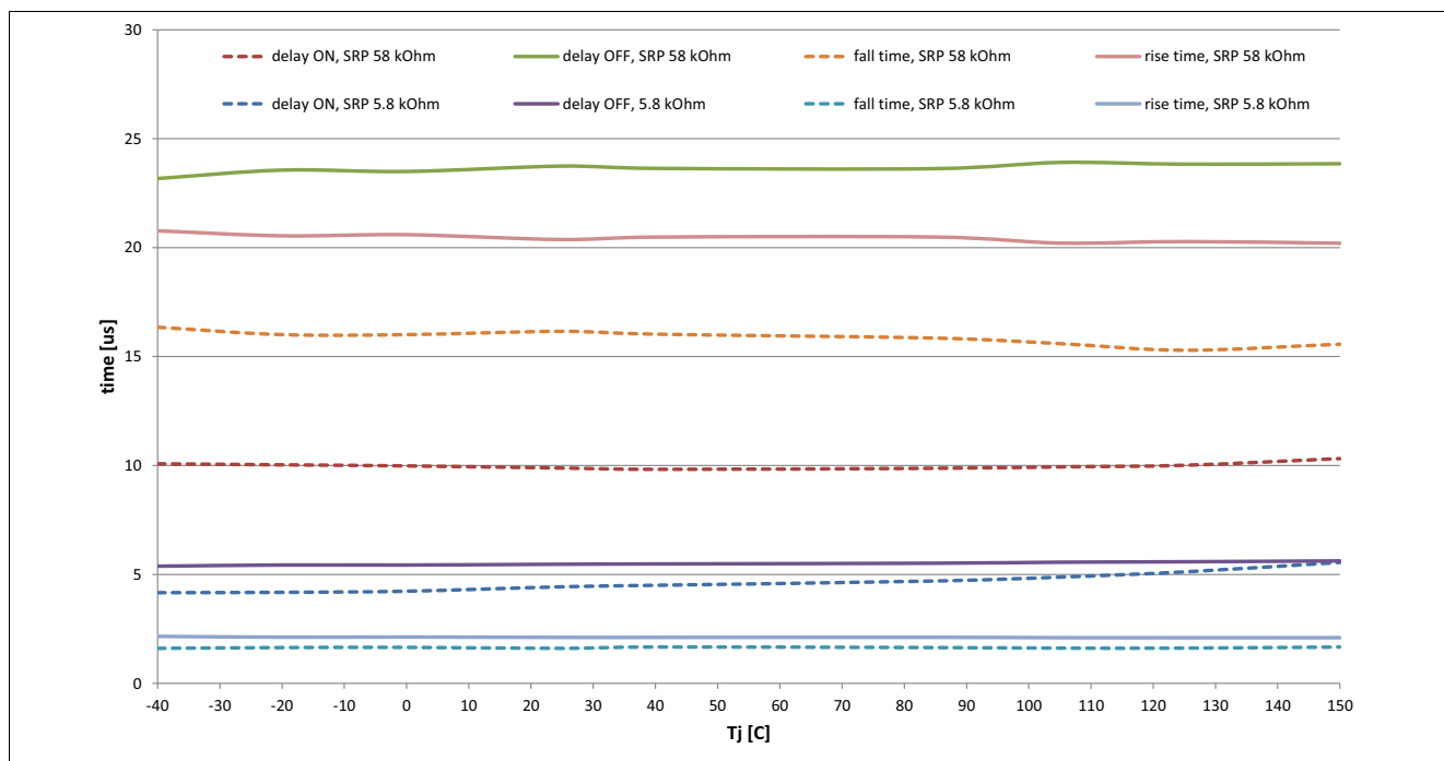
Figure 27 Typical fall time, rise time, delay on time, delay off time vs. T_j (-40..150°C) @ R_{SRP}=5.8k\Omega and 58kΩ) V_{DD}=5V , V_{BAT}=13.5 , V_{IN}=5V
