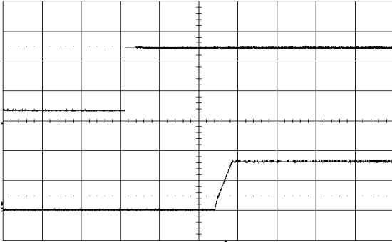
Start-up enabled by connecting V_I at: T_{P1} = +25^\circ\text{C} , V_I = 12\text{ V} , V_O = 3.3\text{ V} C_O = 470\ \mu\text{F}/10\ \text{m}\Omega , I_O = 12\ \text{A} Top trace: Input voltage (5 V/div.). Bottom trace: Output voltage (2 V/div.). Time scale: (20 ms/div.).
