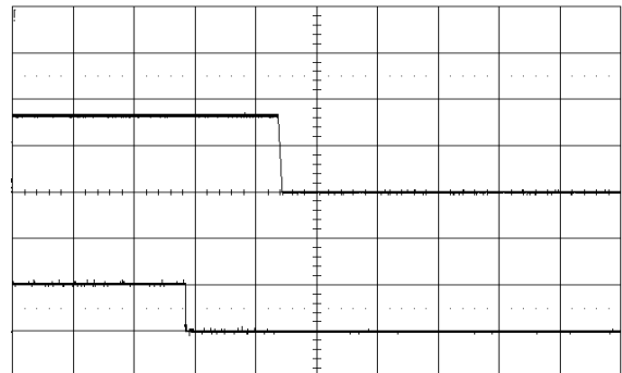
Shut-down enabled by disconnecting V_I at: T_{P1} = +25^\circ\text{C} , V_I = 12\ \text{V} , V_O = 3.3\ \text{V} C_O = 470\ \mu\text{F}/10\ \text{m}\Omega , I_O = 12\ \text{A} Top trace: output voltage (2 V/div.). Bottom trace: CTRL signal (2 V/div.). Time scale: (2 ms/div.).
