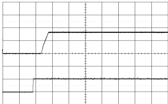
Start-up enabled by connecting V_I at: T_{P1} = +25^\circ\text{C} , V_I = 12\ \text{V} , V_O = 3.3\ \text{V} C_O = 470\ \mu\text{F}/10\ \text{m}\Omega , I_O = 12\ \text{A} Top trace: output voltage (2 V/div.). Bottom trace: CTRL signal (2 V/div.). Time scale: (20 ms/div.).
