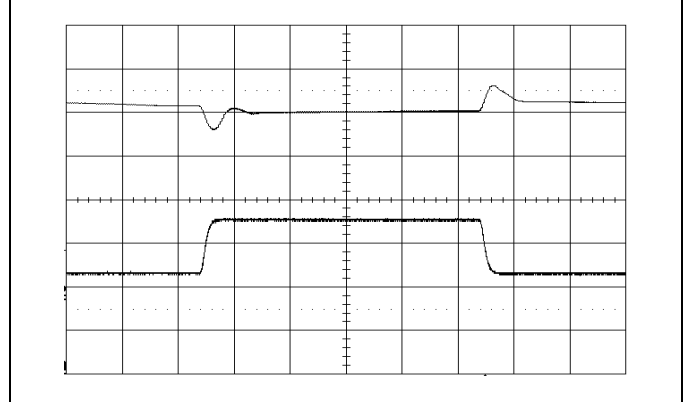
Output voltage response to load current step-change (3-9-3 A) at:
