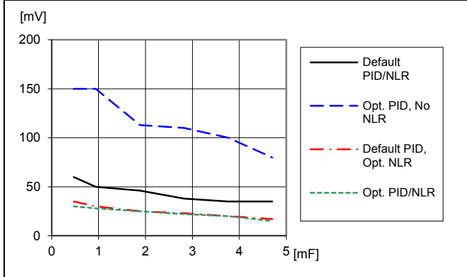
Load transient peak voltage deviation vs. decoupling capacitance. Step-change (3-9-3 A). Parallel coupling of capacitors with 470 \mu\text{F}/10\text{ m}\Omega , T_{P1} = +25^{\circ}\text{C} , V_I = 12\text{ V} , V_O = 1.0\text{ V} , f_{sw} = 320\text{ kHz} , di/dt = 2\text{ A}/\mu\text{s}
