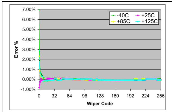
FIGURE 2-56: 50 k \Omega – Worst Case R_{BW} from Average R_{BW} ( R_{BW0} – R_{BW3} ) Error (%) vs. Wiper Setting and Temperature ( V_{DD} = 5.5\text{V} , I_W = 90\ \mu\text{A} ).
