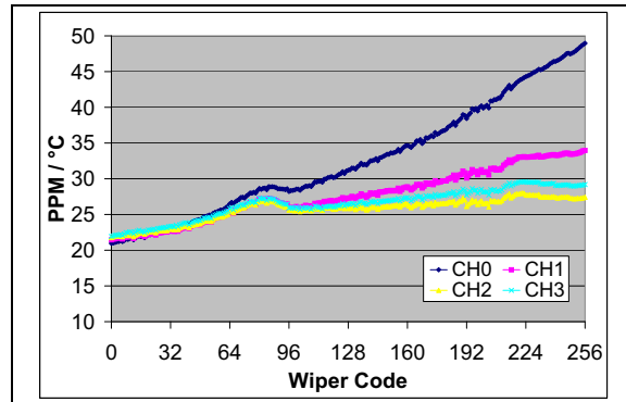
FIGURE 2-39: 10 kΩ – R_{WB} PPM/ ^\circ\text{C} vs. Wiper Setting. ( R_{BW(\text{code}=n, 125^\circ\text{C})}-R_{BW(\text{code}=n, -40^\circ\text{C})})/R_{BW(\text{code} = 256, 25^\circ\text{C})}/165^\circ\text{C} * 1,000,000 ) ( V_{DD} = 5.5\text{V} , I_W = 150\ \mu\text{A} ).
