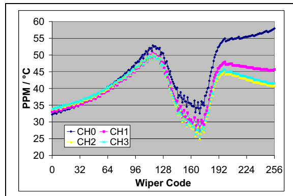
FIGURE 2-40: 10 kΩ – R_{WB} PPM/ ^\circ\text{C} vs. Wiper Setting. ( R_{BW(\text{code}=n, 125^\circ\text{C})}-R_{BW(\text{code}=n, -40^\circ\text{C})})/R_{BW(\text{code} = 256, 25^\circ\text{C})}/165^\circ\text{C} * 1,000,000 ) ( V_{DD} = 3.0\text{V} , I_W = 150\ \mu\text{A} ).
