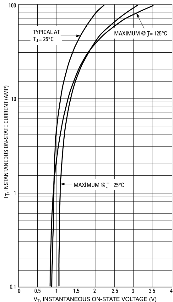
Figure 3. On-State Characteristics
