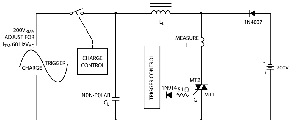
Figure 8. Simplified Test Circuit to Measure the Critical Rate of Rise of Commutating Current ( di/dt )
