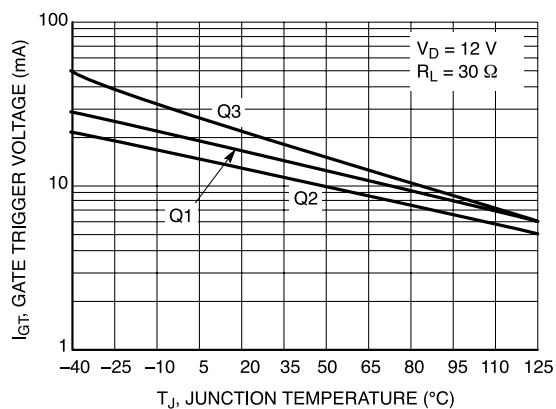
Figure 6. Typical Gate Trigger Current Variation
