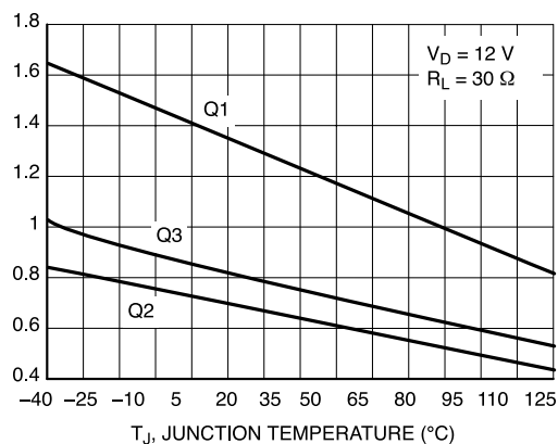
Figure 7. Typical Gate Trigger Voltage Variation
