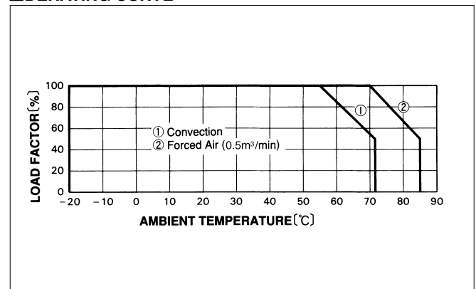
DERATING CURVE
