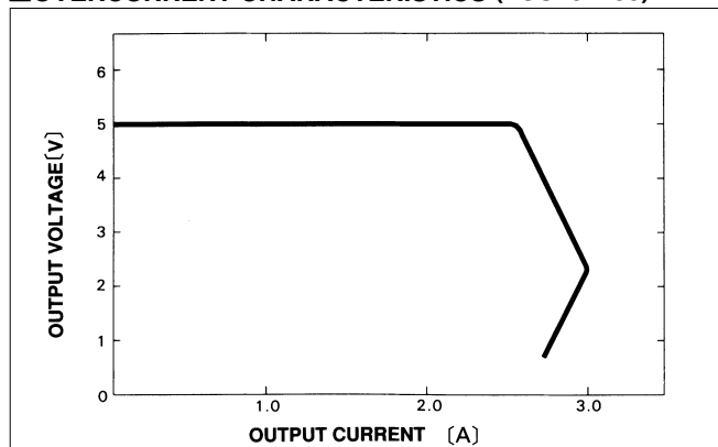
■ OVERCURRENT CHARACTERISTICS (ZUS102405)
