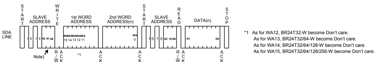
Fig.44 Random read cycle (BR24T32/64/128/256/512/1M-W)
