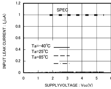
Fig.7 Input leak current I_{L1} (A0,A1,A2,SCL,WP)
