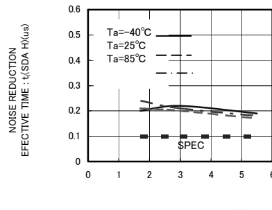
Fig.32 Noise reduction effective time t_i(\text{SDA H})
