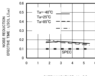
Fig.31 Noise reduction effective time t_i(\text{SCL L})
