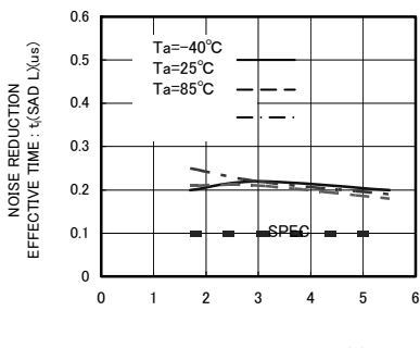
Fig.33 Noise reduction effective time t_i(\text{SDA L})
