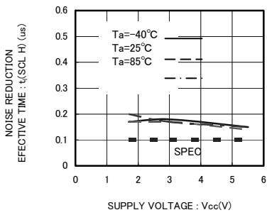
Fig.30 Noise reduction effective time t_i(\text{SCL H})
