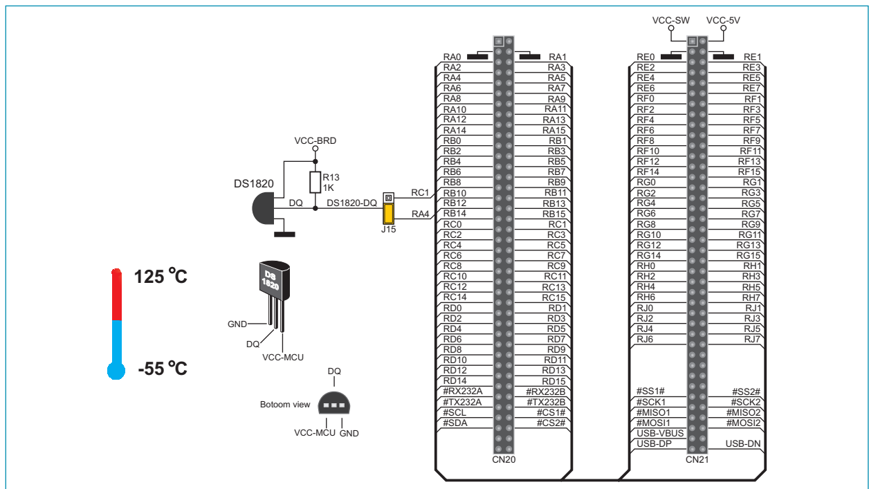
Figure 10-1: DS1820 connector (DS1820 is not connected)
