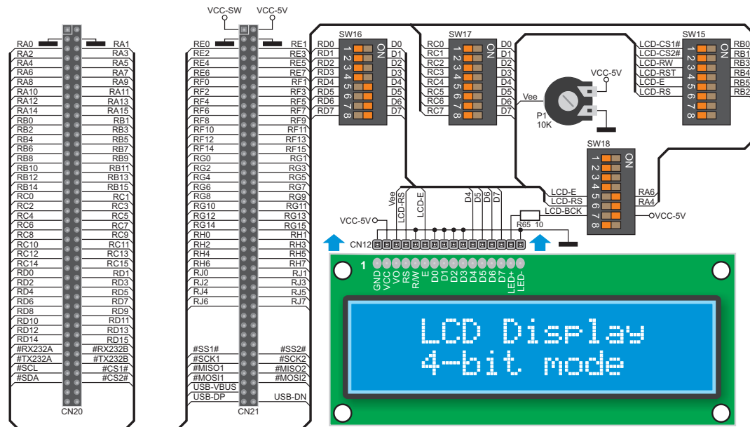
Figure 14-3: 2x16 LCD display connection schematic
