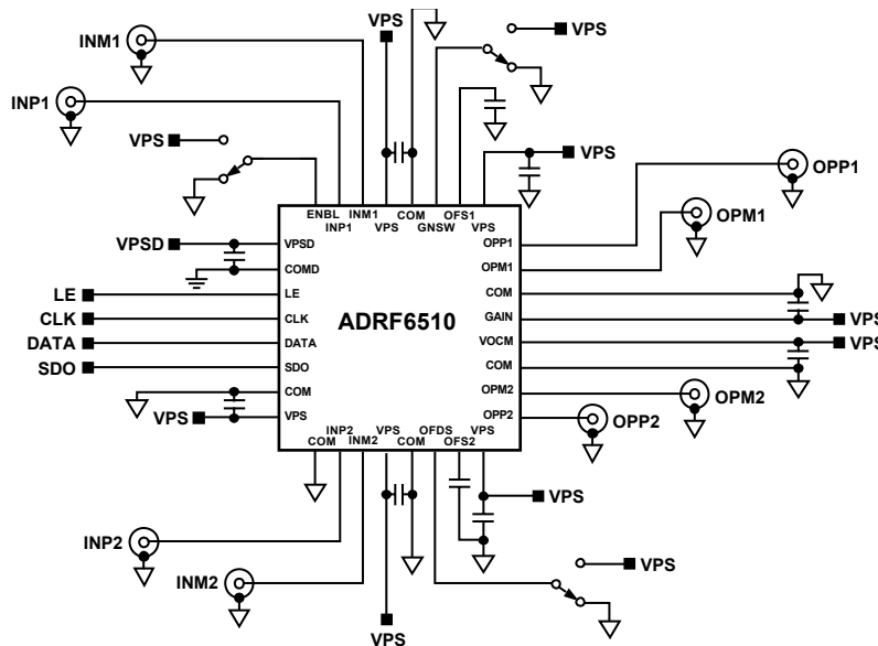
Figure 49. Basic Connections
