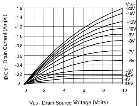
Saturation Characteristics
