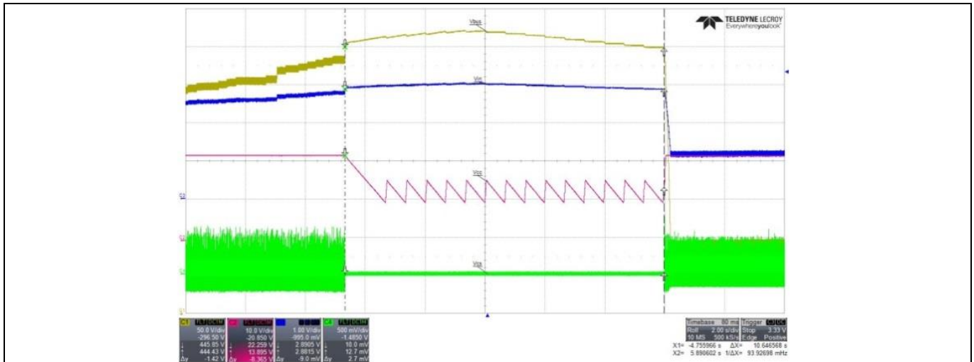
C1 (yellow): V_{BUS} ; C2 (purple): V_{CC} ; C3 (blue): V_{IN} ; C4 (green): V_{CS}
