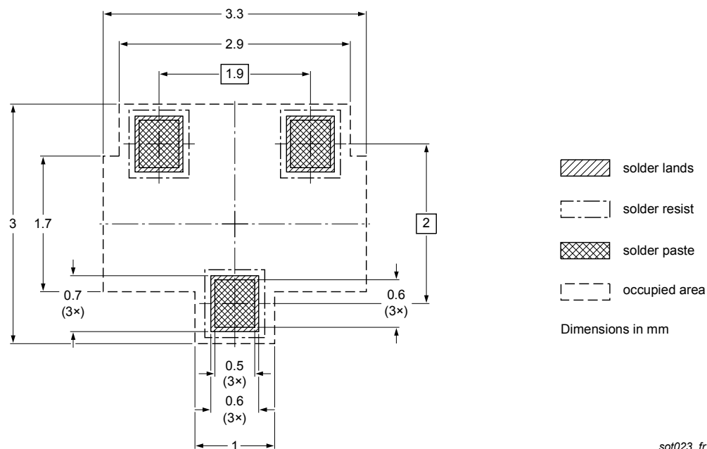
Fig. 28. Reflow soldering footprint SOT23 (TO-236AB)
