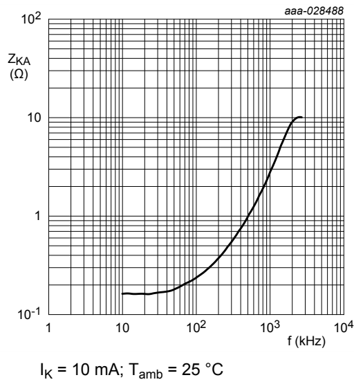
Fig. 15. Dynamic cathode-anode impedance as a function of frequency; typical values
