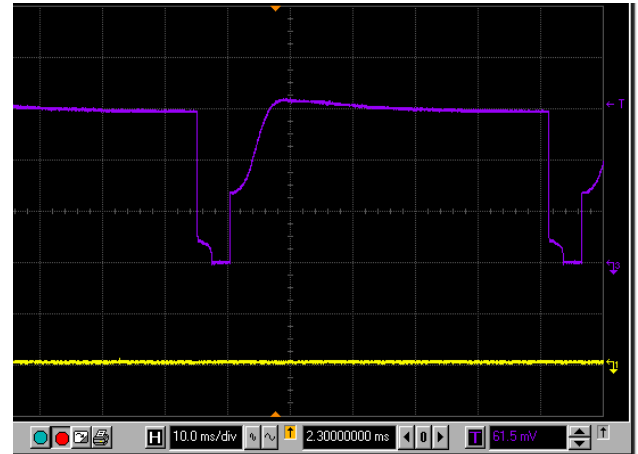
FIGURE 17. THE ISL9491 ENTERING THERMAL SHUTDOWN WITH R_{ILIM} = 0
