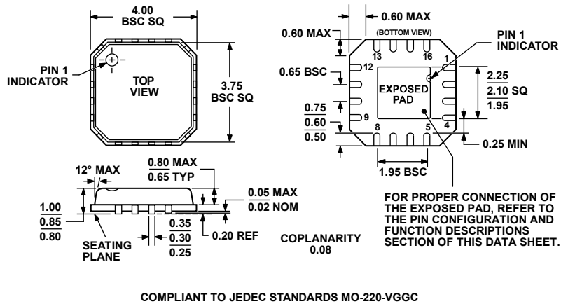
Figure 43. 16-Lead Lead Frame Chip Scale Package [LFCSP_VQ] 4 mm x 4 mm Body, Very Thin Quad (CP-16-4)
