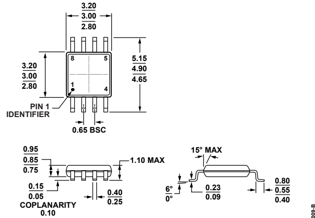
Figure 42. 8-Lead Mini Small Outline Package [MSOP] (RM-8)
