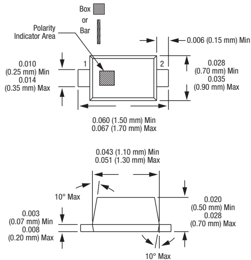
Dimensions are in inches (millimeters shown in parentheses) 200049-008
