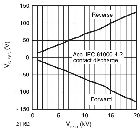
Fig. 9 - Typical Clamping Voltage at \pm ESD Contact Discharge (acc. IEC 61000-4-2)
