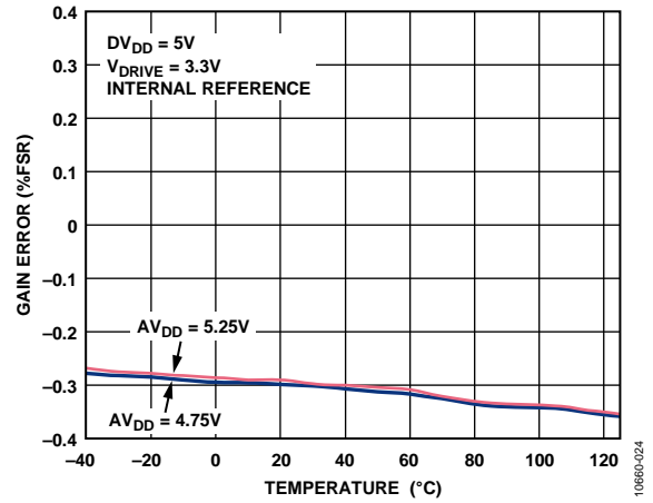
Figure 25. DAC Gain Error vs. Temperature
