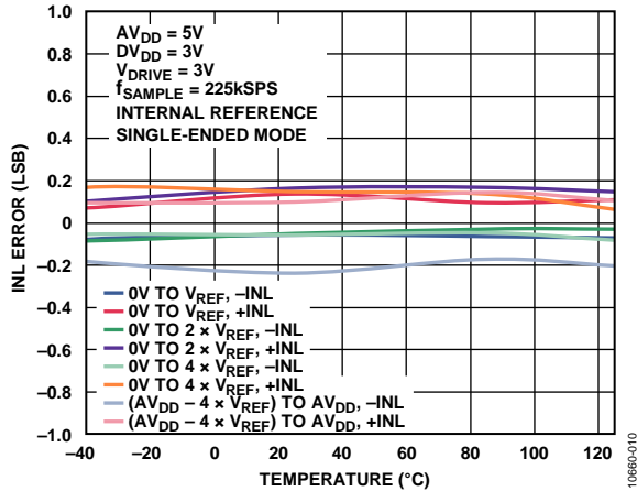
Figure 10. ADC INL vs. Temperature
