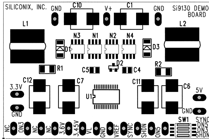
FIGURE 1. Top Silkscreen
