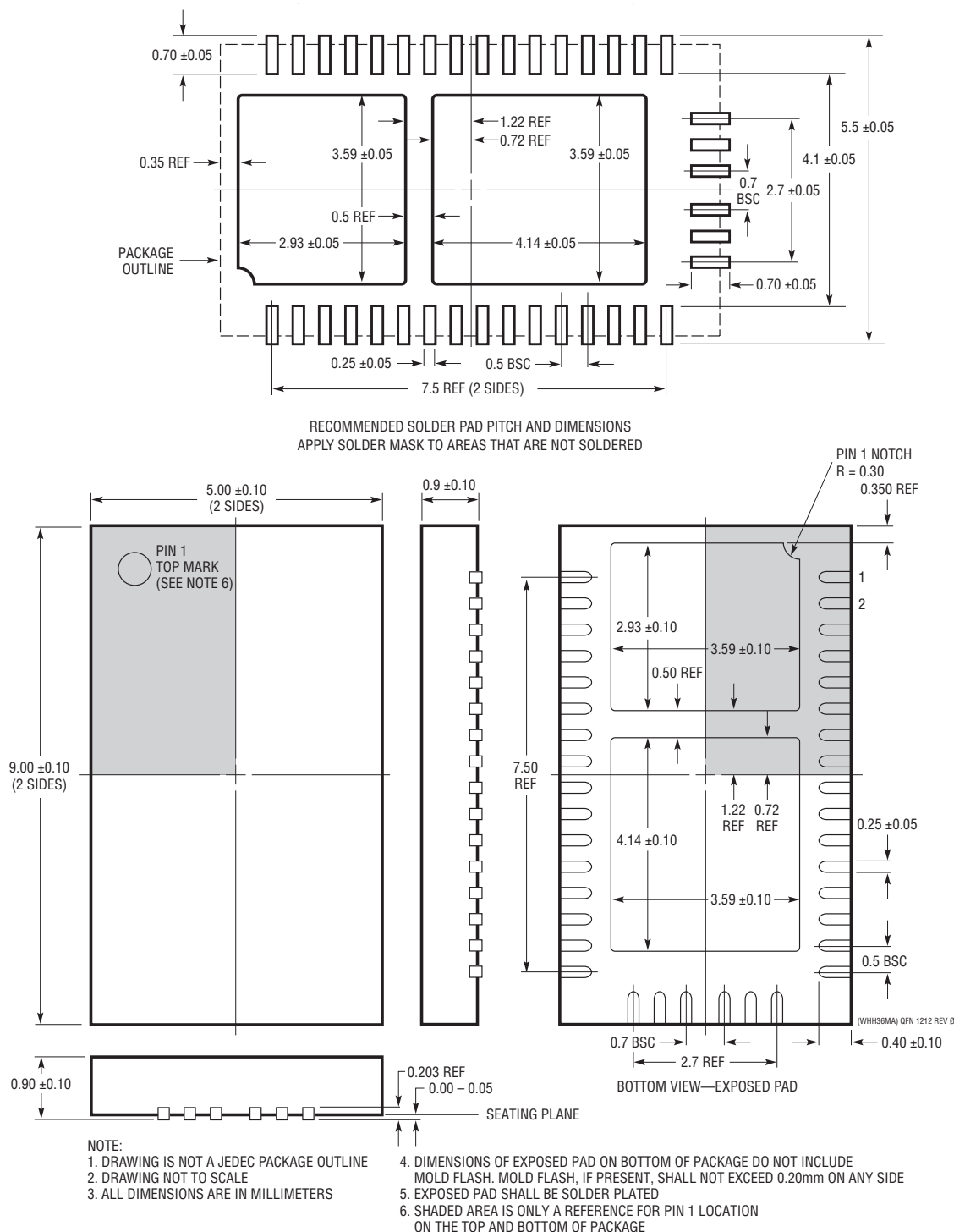
WHH Package Variation: WHH38MA 38-Lead Plastic QFN (5mm x 9mm) (Reference LTC DWG # 05-08-1934 Rev 0)
