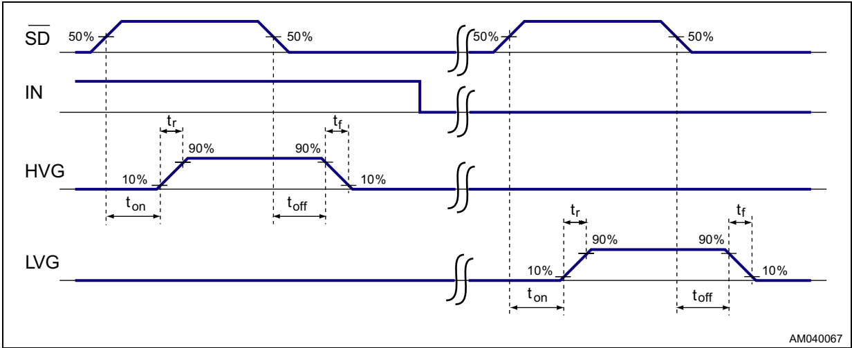
Figure 3. \overline{SD} timings
